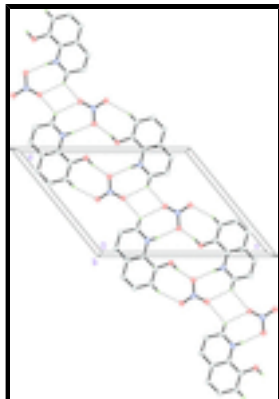
Fig. 2. The crystal structure of the title compound, viewed along the b axis.
